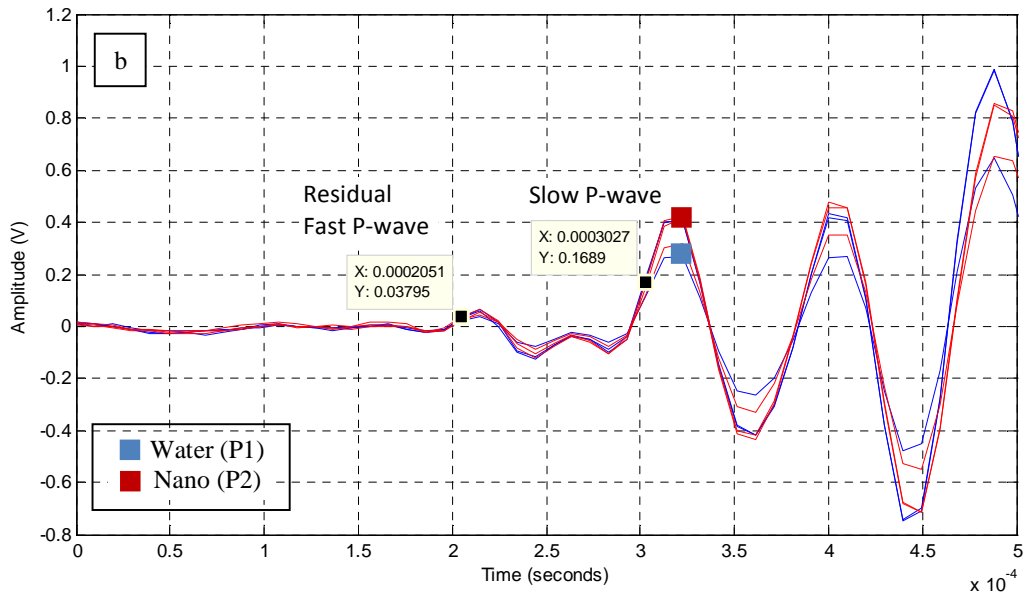
Figure 8.21. 8 kHz sine pulse with 200 Hz high-pass filter applied in saturated glass bead specimen for testing differences in compression with water and nAg at 3.7% dispersion, showing three repetitions of 1000 recordings averaged per repetition.
