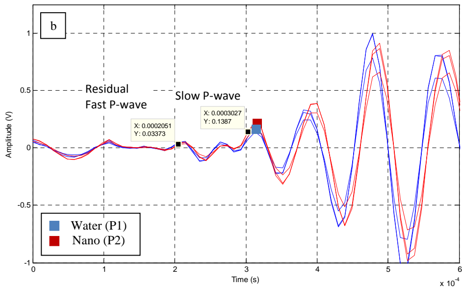
Figure 8.17. 8 kHz sine pulse with 200 Hz high-pass filter applied in saturated glass bead specimen for testing differences in compression with water and nTiO 2 at 4.9% dispersion, showing three repetitions of 1000 recordings averaged per repetition.
