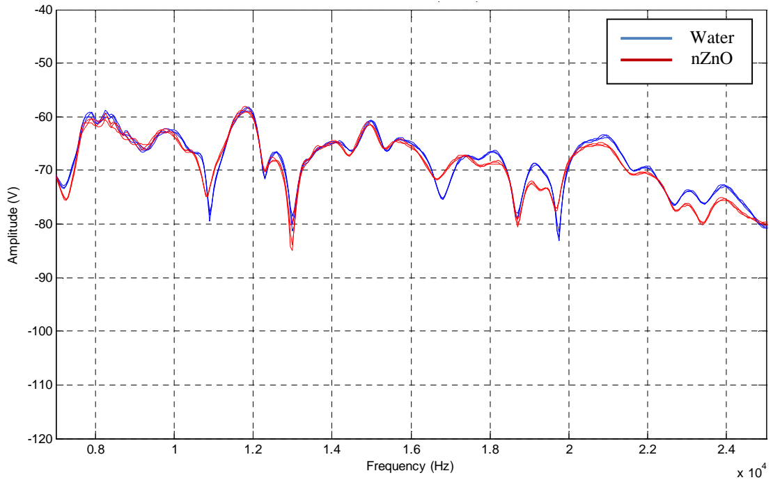
Figure 8.11. 30 kHz sweep with 200 Hz high-pass filter, testing spectral response in a saturated glass bead specimen in water and in the presence of nZnO at 0.3% dispersion, showing three repetitions of 1000 recordings averaged per repetition.
