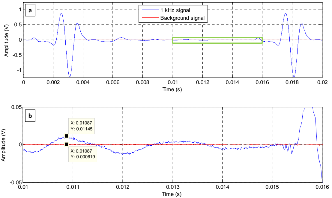
Figure A3.2. 1 kHz sine pulses (200 Hz high-pass filter) overlaid on the isolated background signal (no filter). Each signal is a single repetition of 1000 recordings averaged.
